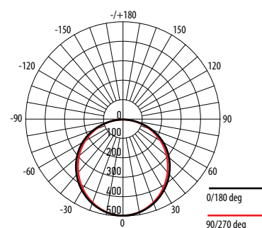
PPO 1200/L SMD 40W 6500K
